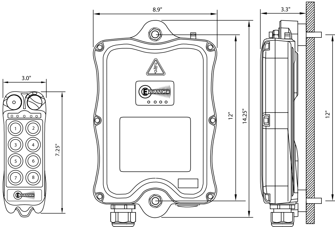
TYPICAL TRANSMITTER LAYOUT
